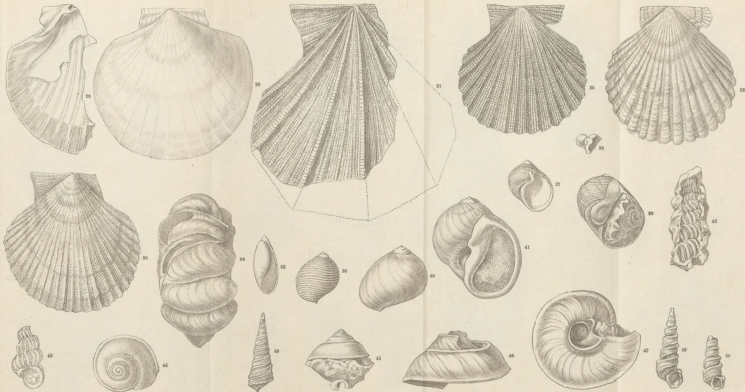
28-29 Pecten Darwinii 30 " Parrensis d'Orbig 31 " centralis 32 " rudis 33 " actinoides 34 Crepidula gregaria 35 Bulla cosmophila 36-37 Sigaretus subglobosus 38 Natica pumila 39 Natica striolata 40-41 " solida 42-43 Scalaria rugulosa & var 44-45 Trochus collaris 46-47 Trochus laevis 48 Turritella Patagonica 49 " ambulacrum 50 " suturalis
