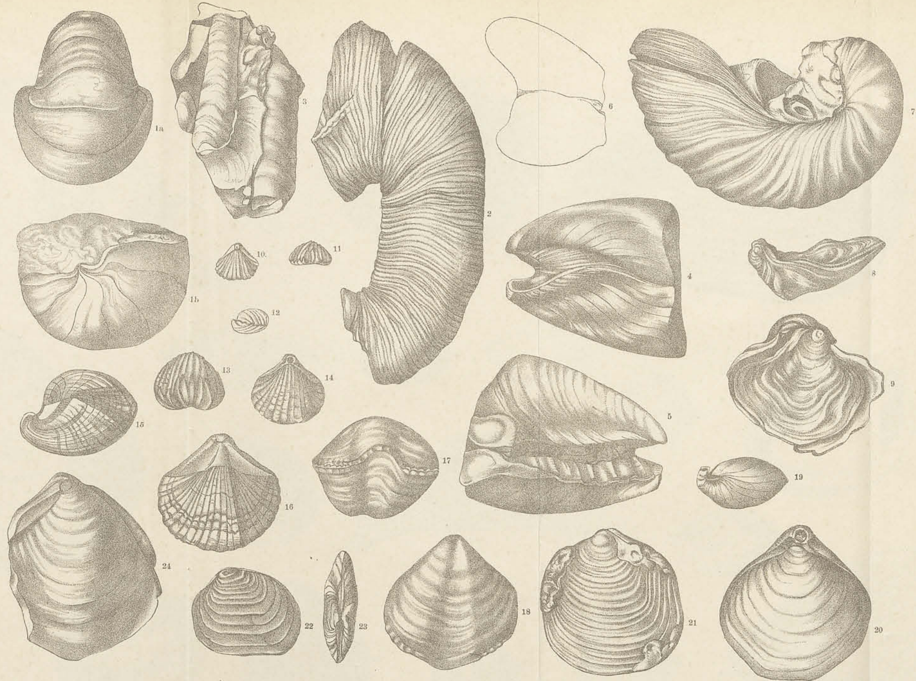
1a-1b Nautilus d'Orbignyanus 2 Ancyloceras simplex 3 Baculites vagina 4, 5, 6, Perna Americana 7 Gryphæa Darwinii 8, 9 Gryphæa nov. spec. 10, 11, 12 Terebratula enigma 13, 14 var. of do 15, 16 Spirifer Chilensis 17, 18 " linguiferoides 19, 20 Terebratula inca 21 Lucina excentrica 22, 23 Astarte Darwinii 24 Lucina Americana
